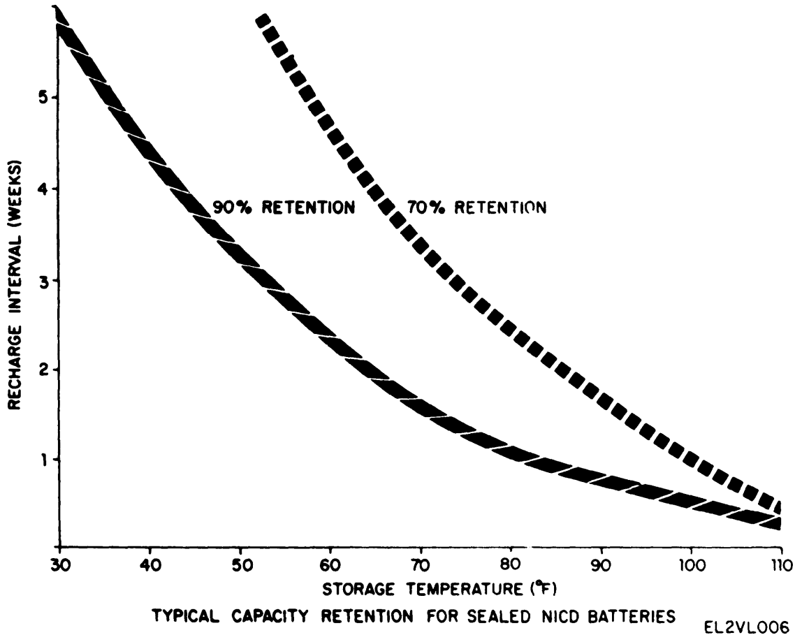
Figure 2-3. Typical Capacity Retention for Sealed NiCD Batteries
