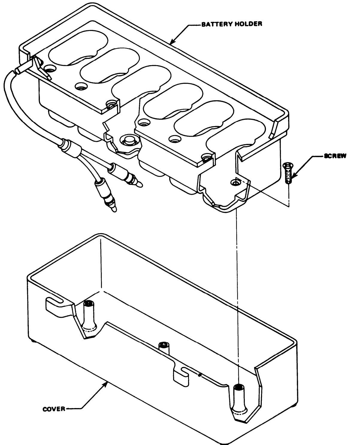
Figure 1-1.1. Battery Charging Tray Assembly MX-10154( )/U
